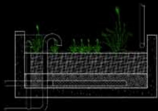
S3 RAIN PLANTER
