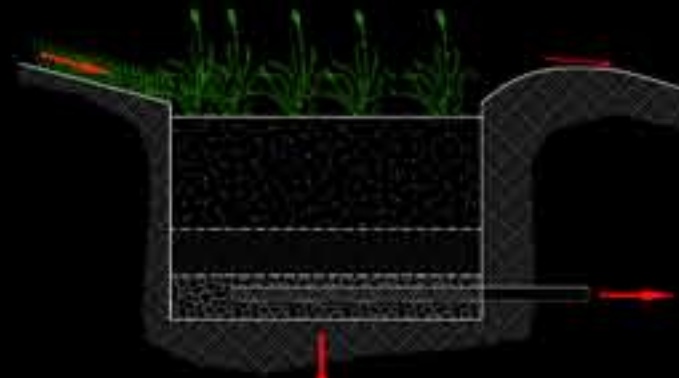
S4 RAIN GARDEN
