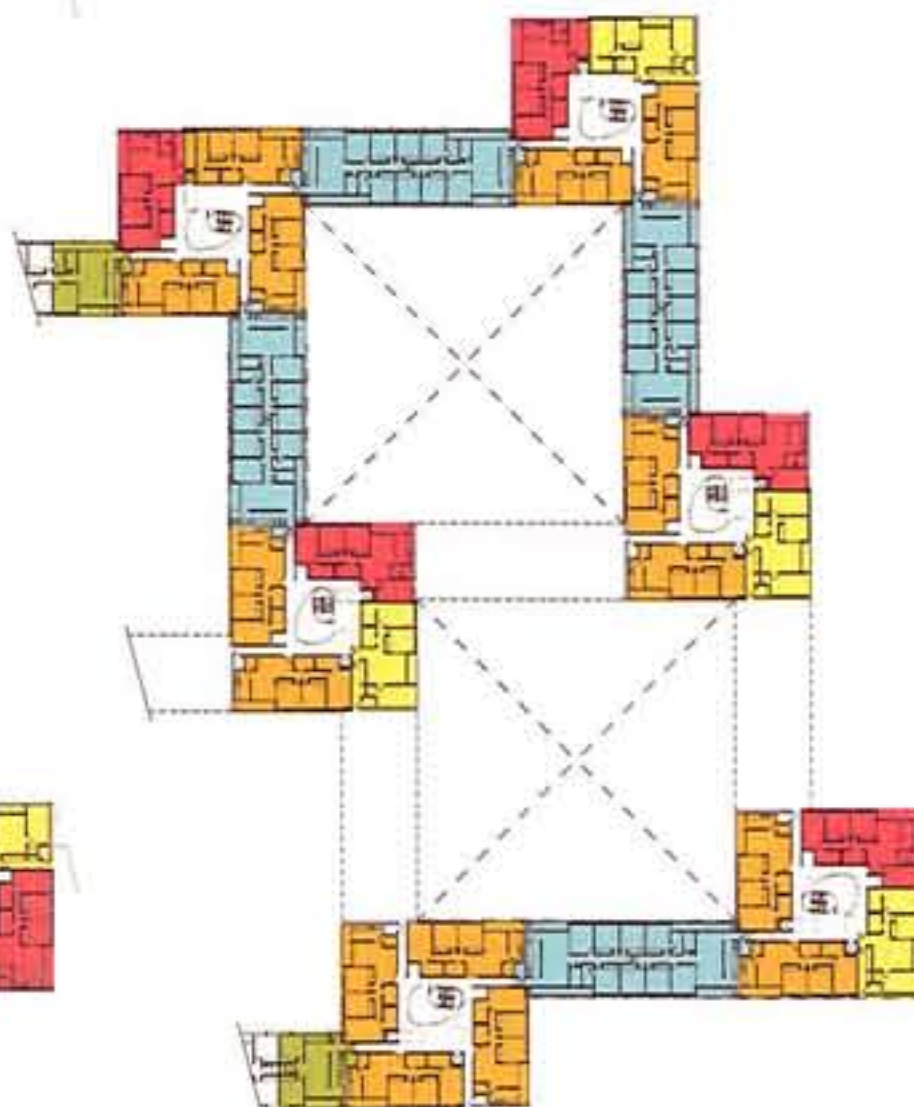
4TH TO 7TH STOREY PLAN - SCALE 1:750
