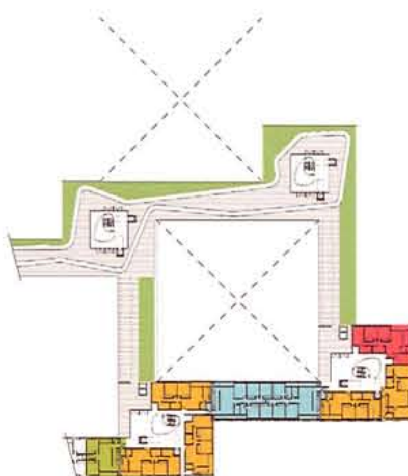
14TH TO 18TH STOREY PLAN - SCALE 1:750
